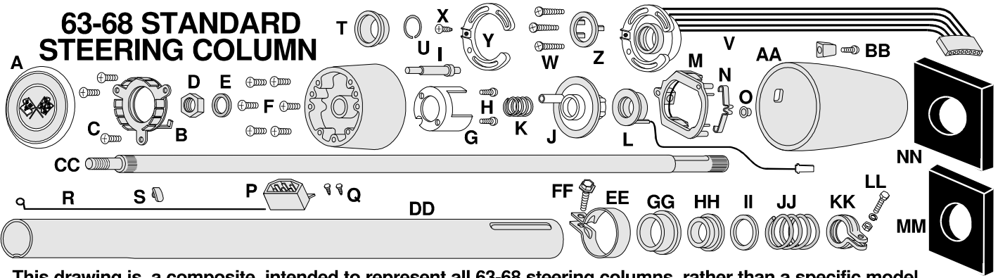
This drawing is a composite, intended to represent all 63-68 steering columns, rather than a specific model.
